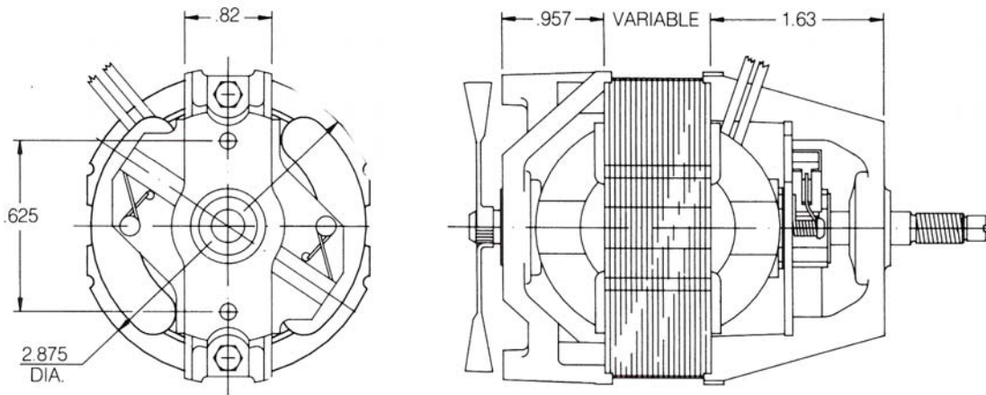
Totally enclosed or skeleton frame motors
